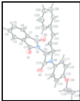
Fig. 1. View of the molecular structure of (I), with 30% probability displacement ellipsoids for the non-hydrogen atoms.
