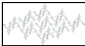
Fig. 2. View of the packing and hydrogen bonding interactions for (I). H atoms not involved in hydrogen bonding have been omitted for clarity.
